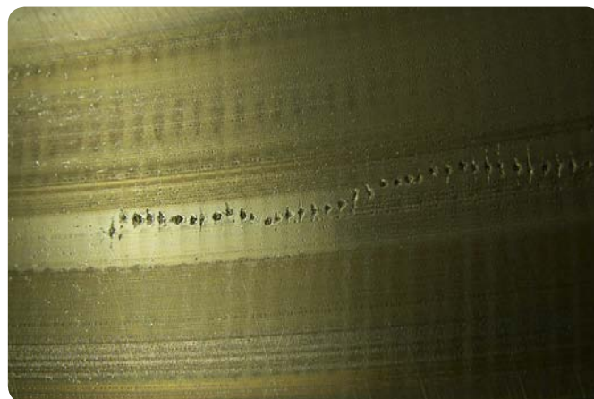
Spherical roller bearing – roller Enlarged view of craters in a bead-like formation
