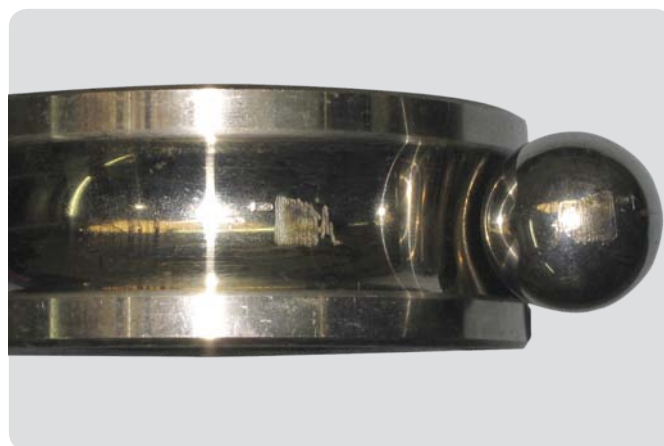
Deep groove ball bearing inner ring and ball Excessive current resulting in a number of craters in zig-zag formation on the ball and raceway
